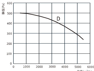
QFA-D5000P (-Y) 性能曲线图
